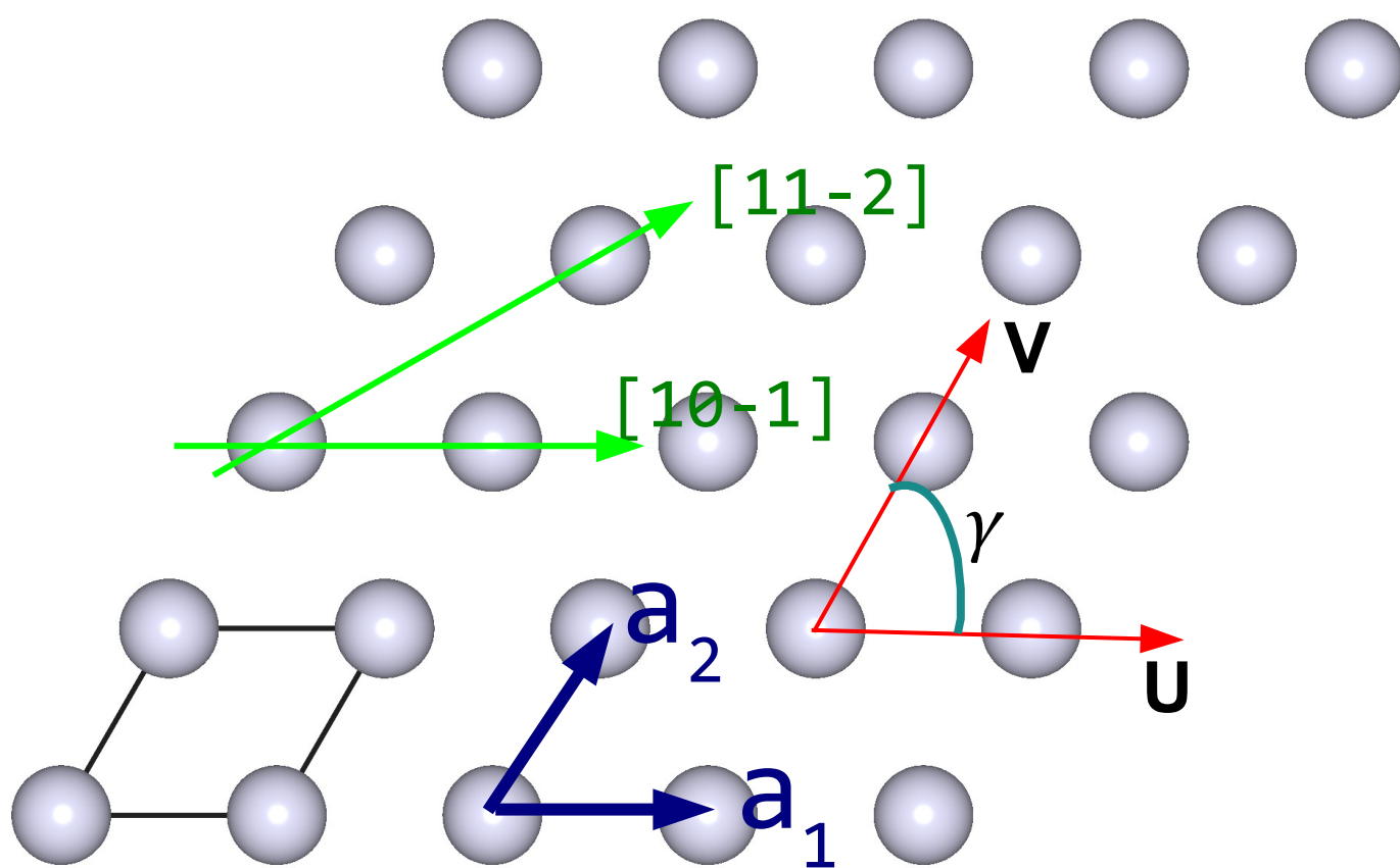
Direct lattice
