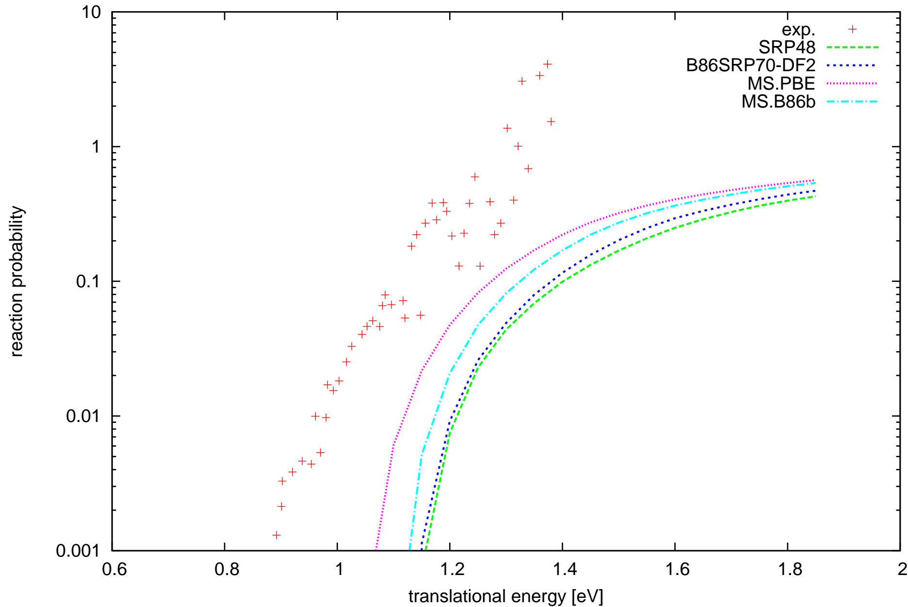
H 2 + Ag(111) -- v 0 J 3 degeneracy averaged
