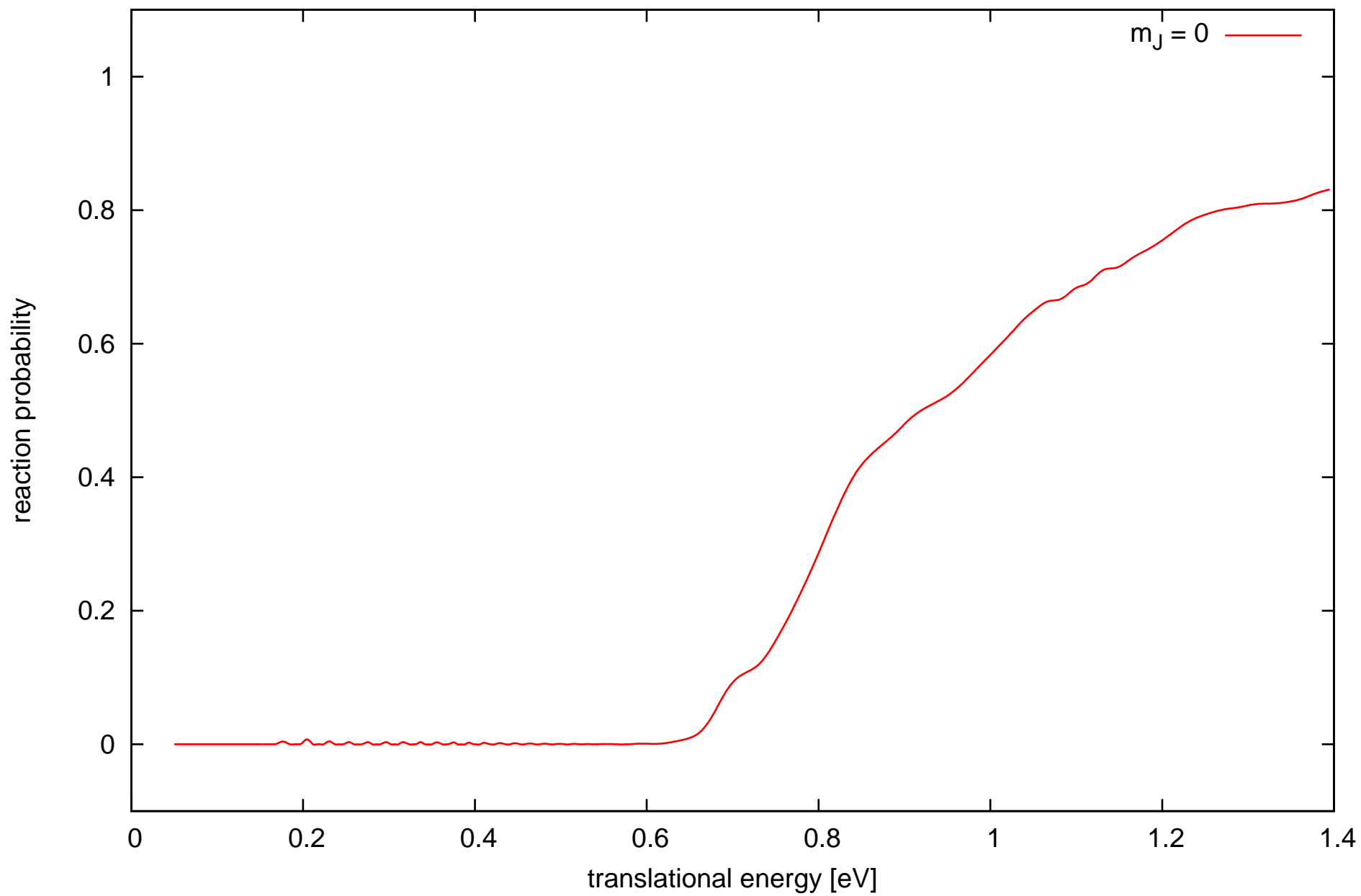
QD Cu(111) -- state v = 0 J = 0
