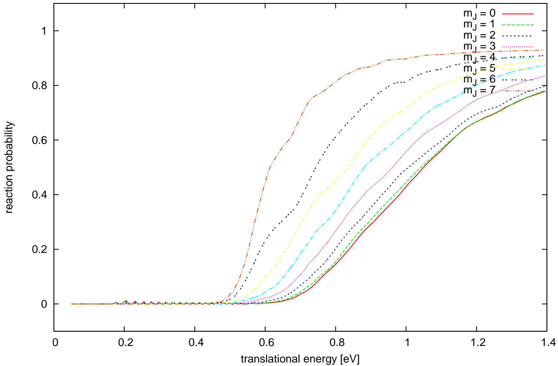
QD Cu(111) -- state v = 0 J = 7
