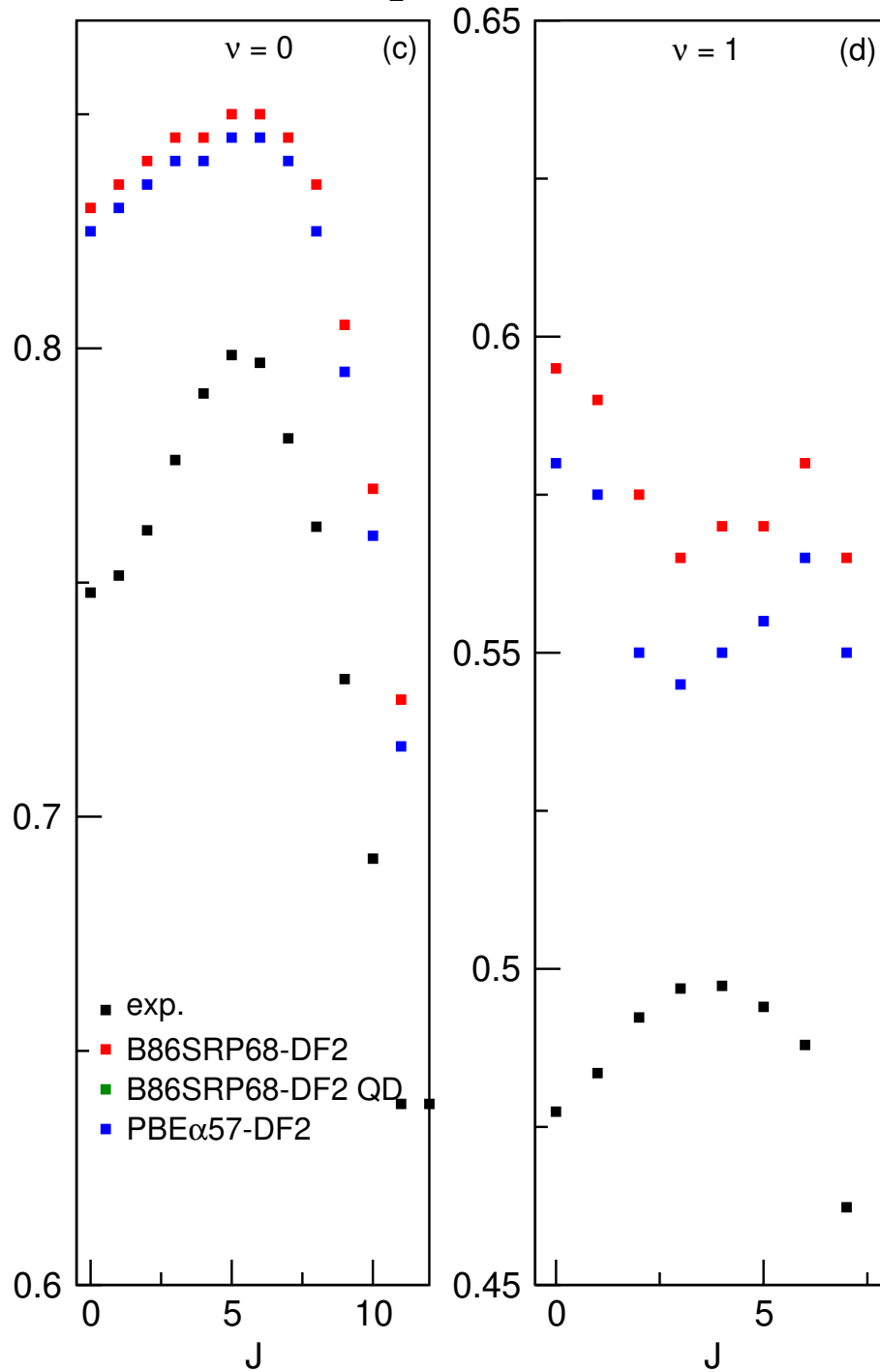
\text{D}_2 + \text{Cu}(111)
