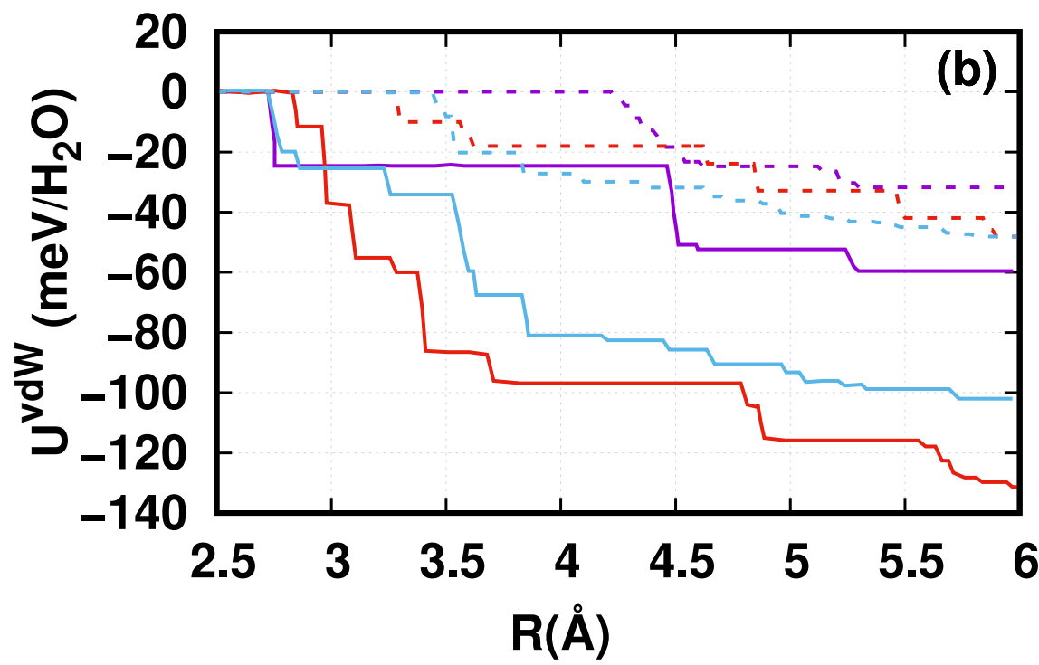
PBE+TS and TIP4P/2005
